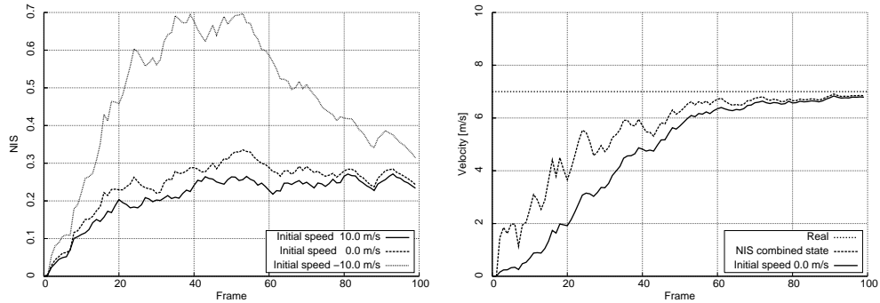
(a) Low pass filtered normalized innovation squared of the filters from figure 2(b).
